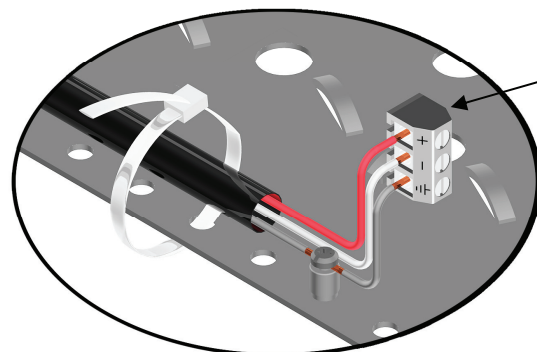
STICK-ON Module Terminal Block
